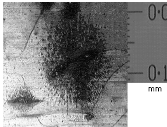
Figure 37 Smoothly curved lines and radial lines coming out of a primary crater on the an aluminum cathode
